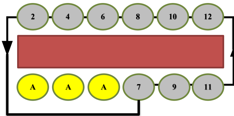
Figure 3 Rotation for even number of players, 3 anchors
